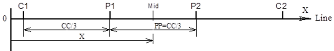
Slika 14. Wenner-ov raspored
